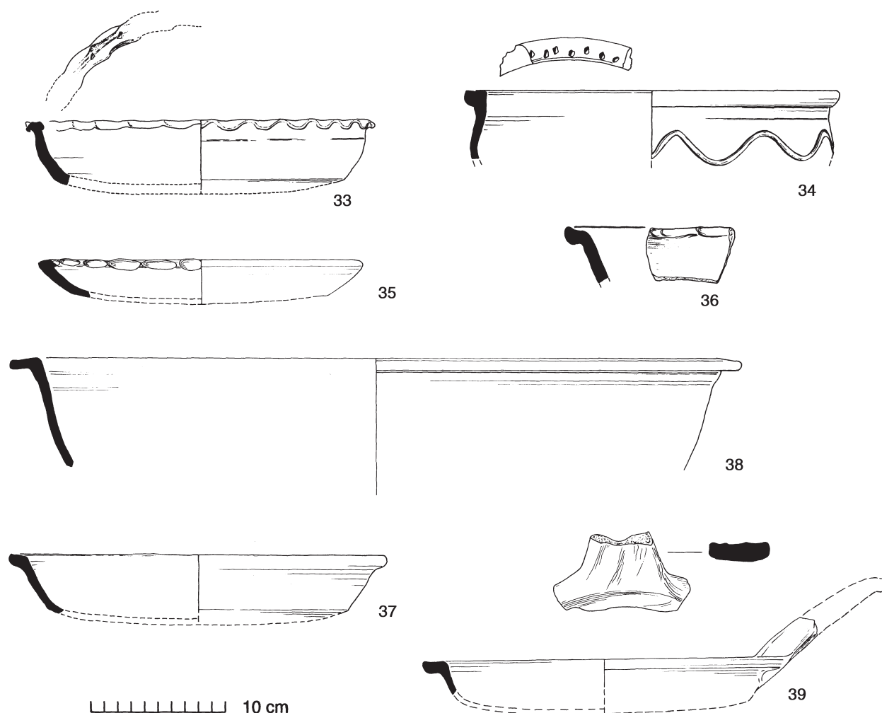
Fig 62 Medieval greyware: bowls (nos 33-38); frying pan (no 39). 1:4.
