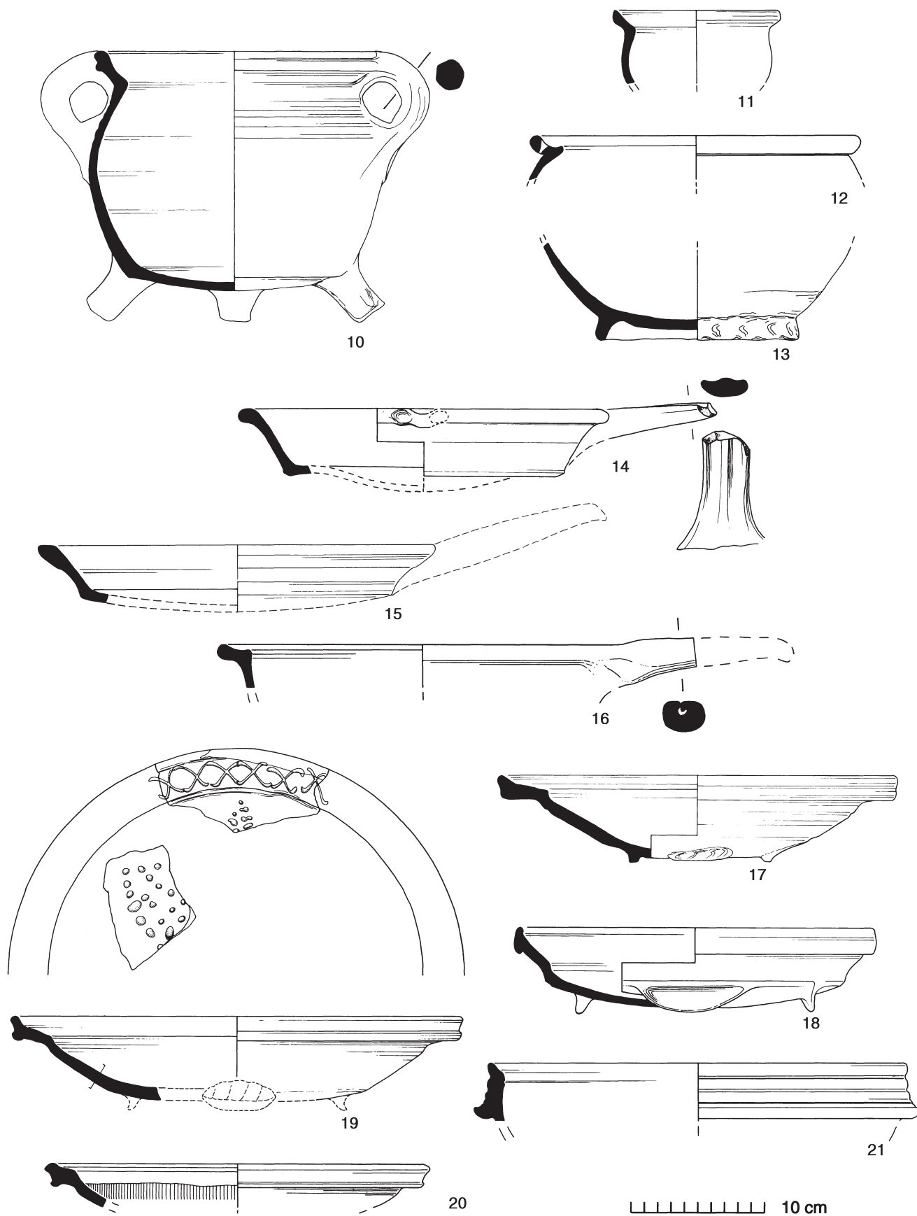
Fig 180 Low Countries red earthenwares: cauldron (no 10); miscellaneous jars (nos 11-13); skillets (nos 14-16); dishes and bowls (nos 17-21). 1:4.
